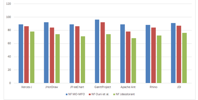
Fig. 8. Median percentage of fixed code smells (NF) on the different pull-requests of the seven systems.
